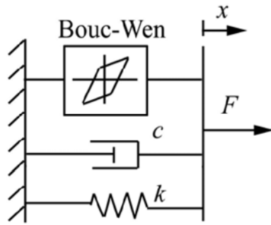
Fig. 4. Bouc-Wen model.
