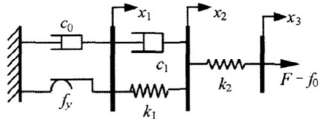
Fig. 3. Bingham model.
