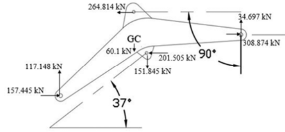
Figure 11. Forces applied on the boom.
